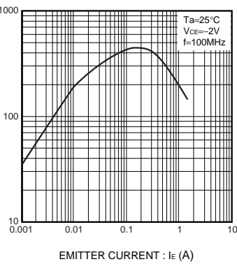
Fig.6 Gain bandwidth product vs. emitter current
